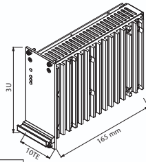
Standard Eurocassette (pluggable module for 19" sub-rack) approx. 0.7 kg
