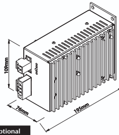
Optional Chassis mount approx. 1.05 kg
