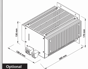
Optional Chassis mount (available for currents up to 60Amps) approx. 4.6 kg
