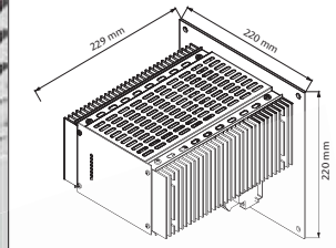
Optional Wall mount approx. 6.0 kg
