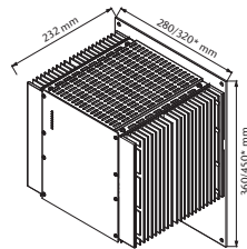
Optional Wall mount approx. 16 kg / *) 19 kg *) applicable to models >= 150 A output current
