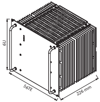
Standard Eurocassette (pluggable module for 19" sub-rack) approx. 13.0 kg
