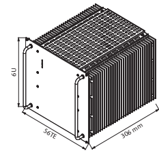
Standard Eurocassette (pluggable module for 19" sub-rack)
