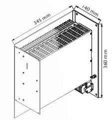
Optional Wall mount approx. 13.0 kg
