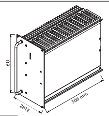
Standard Eurocassette (pluggable module for 19" sub-rack) approx. 9.0 kg
