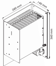
Optional Wall mount approx. 9.5 kg
