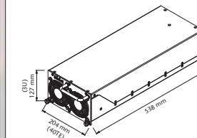
Standard Pluggable module (for 3U sub-rack) approx. 17 kg
