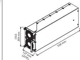
Standard Pluggable module (for 5U sub-rack) approx. 17 kg
